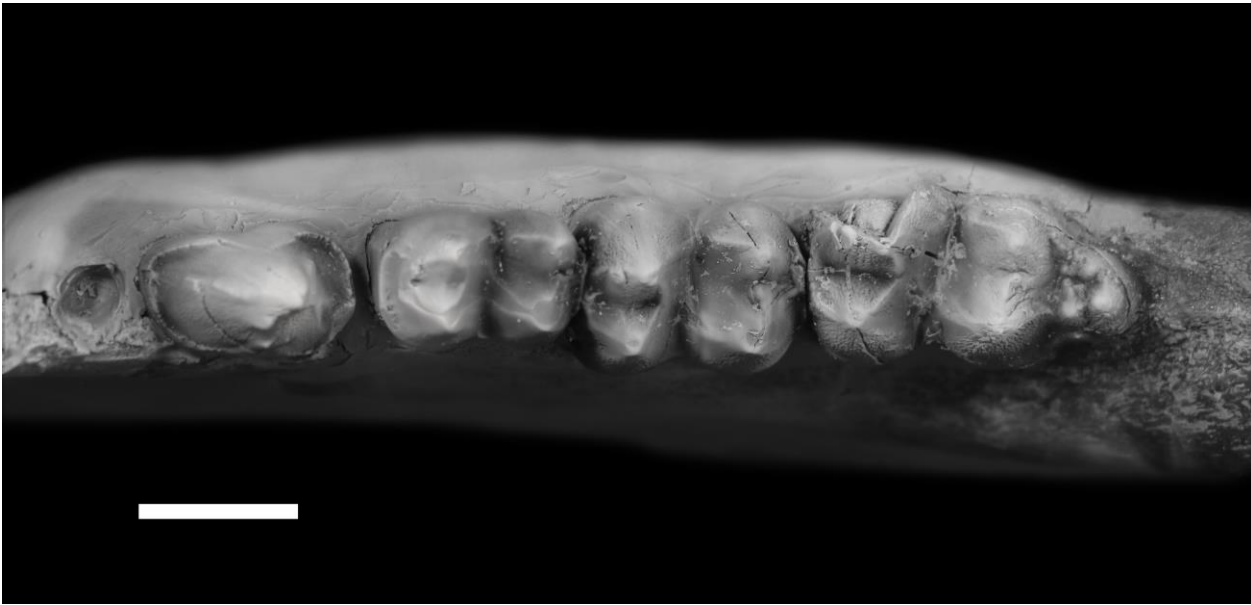
FIGURE 2. Heliosus apophis FHPR 13976. Occlusal view of dentition. Scale bar equals 1 cm.
